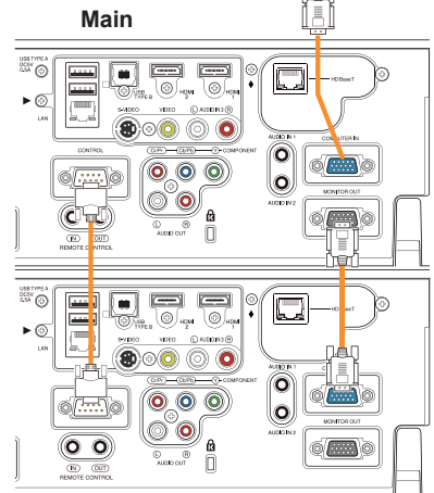
Sub Connection example in Intellectual Stack
